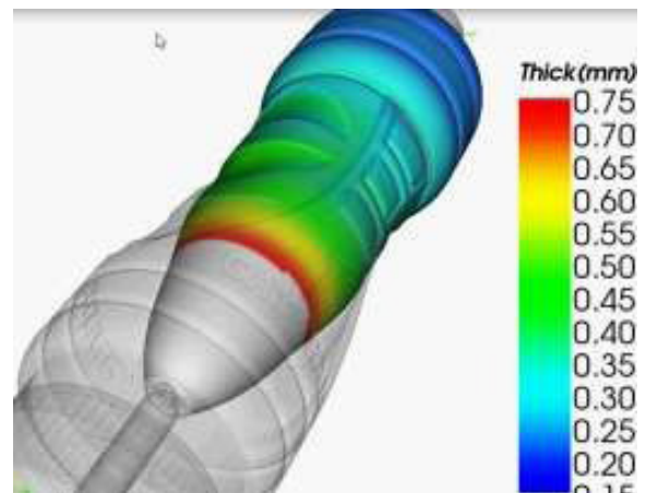
Ever wondered what the inside of a blow mold or injection mold look like during filling? With Abaqus, you can visualize exactly what’s going on.
