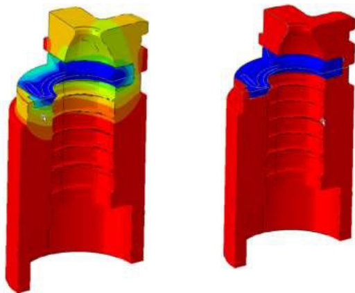
Abaqus can also be used to simulate the manufacturing process. Here, the effects of inadequate mold insulation are easily visualized—on the left is a tool with no insulation, while the right shows one that’s been fully insulated.
