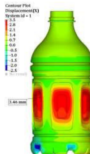
This Abaqus simulation clearly illustrates side panel displacement when a rigid plastic bottle is subjected to pressure.
