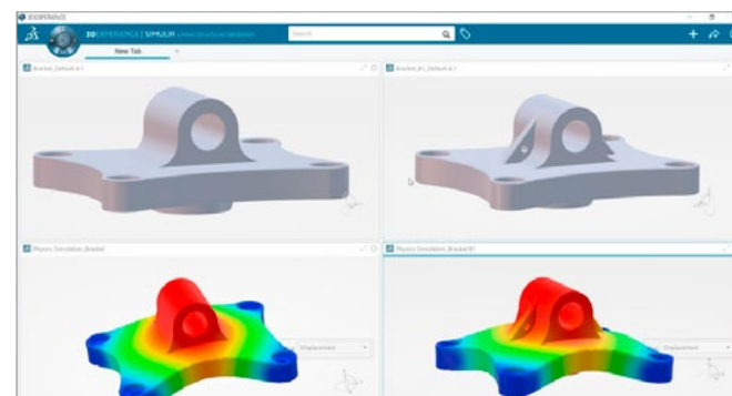
Structural Simulation
